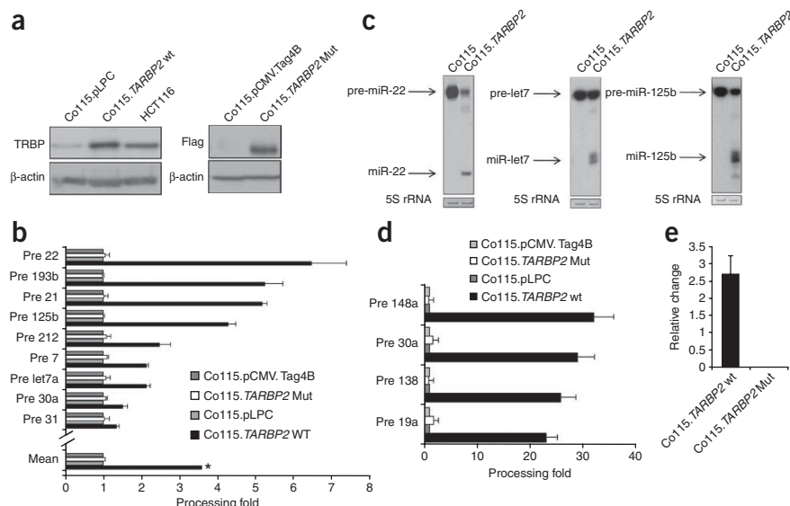
Figure 2 Transfection of wild-type TARBP2 rescues pre-miRNA processing capacity. (a) TRBP protein expression was restored after transfecting wild-type TARBP2 in Co115 cell line. Stable clones were selected treating cells with puromycin (left). As a control, the truncated form of TARBP2 , due to the mutation in the (C) 5 repeat, was also transfected in a pCMV-Tag4b vector and tested using an antibody against Flag. Stable clones were selected using G418. (b) Co115 cell line transfected with wild-type TARBP2 presented a 3.6-fold increase in the capacity of processing the existing precursor miRNAs compared with cells transfected with empty vector. No changes were observed in cells transfected with the TARBP2 truncated form in comparison to cells transfected with empty vector. * P < 0.001. (c) RNA blot analysis confirmed a defect in the generation of mature miRNAs in TARBP2 mutant Co115 cells that was rescued by transfection of wild-type TARBP2 . (d) Synthetic precursor molecules were transiently transfected in Co115 cells that stably expressed TARBP2 wild-type and truncated form, versus cell lines transfected with empty vector. Only in Co115 cells transfected with wild-type TARBP2 did we observe an increase in the capacity to process the transfected precursor molecules. ** P < 0.005. (e) The use of a miRNA microarray platform showed an increase in the number of overexpressed mature miRNAs in the Co115 TARBP2 -transfected cells, whereas transfection of the TARBP2 mutant form did not cause any miRNA overexpression. Error bars, s.e.m.
